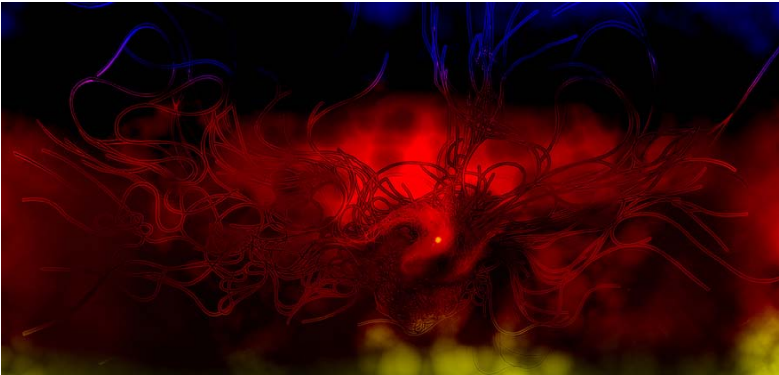
Airplane-After
